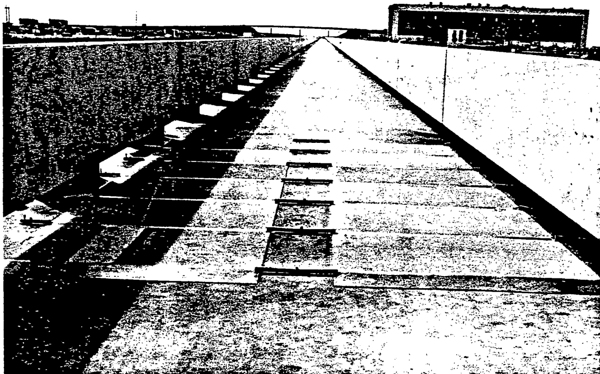
Figure 6. Surface Irregularities in TLRV Guideway to Study Vehicle Response and Behavior.
