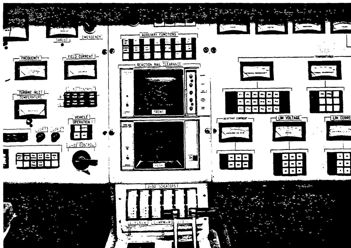
Figure 12. LIMRV Instrument Van Remote Control Panel.
