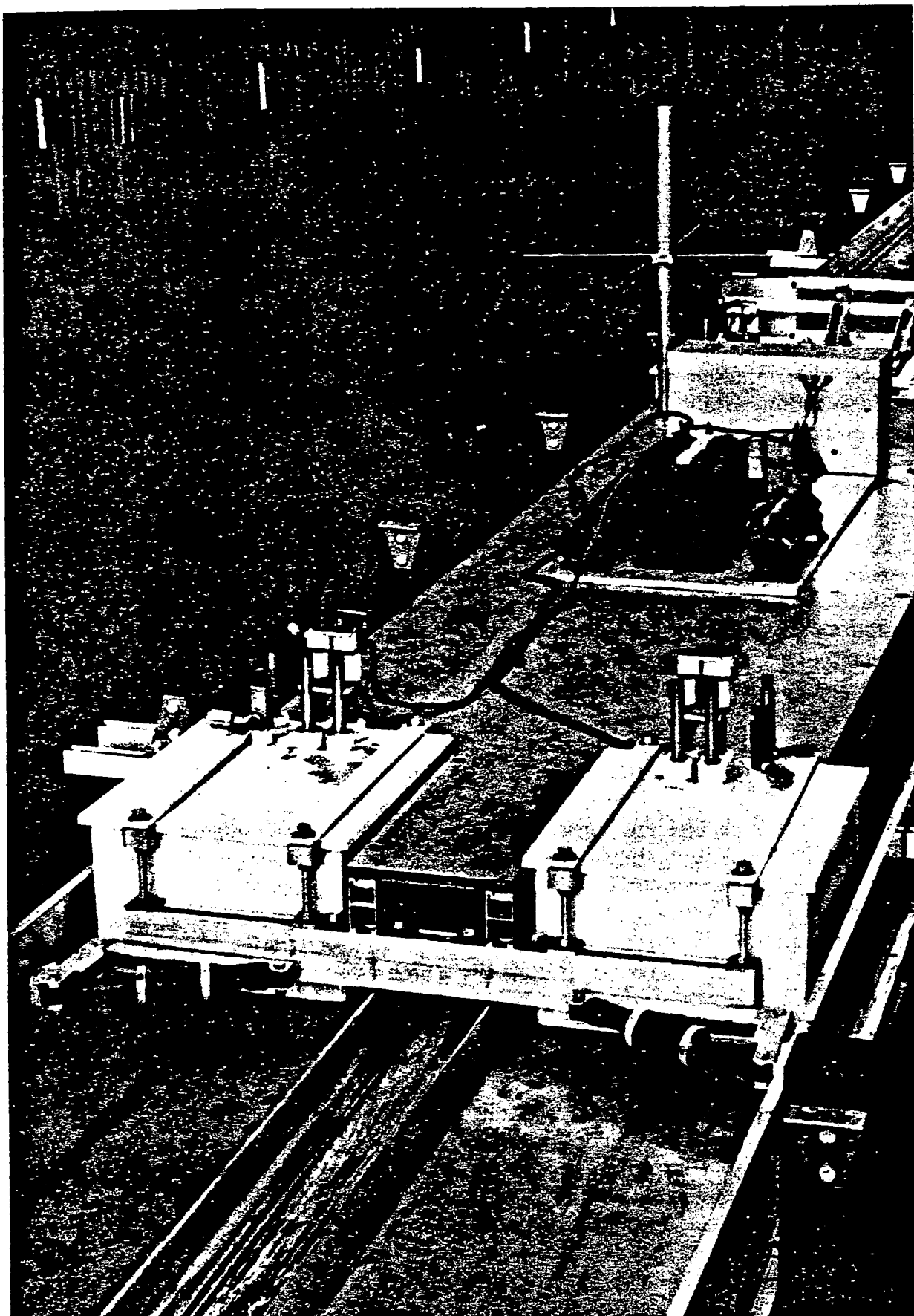
Figure 9. Magnetically Levitated Test Vehicle on Aluminum Guideway (Repulsive System).
