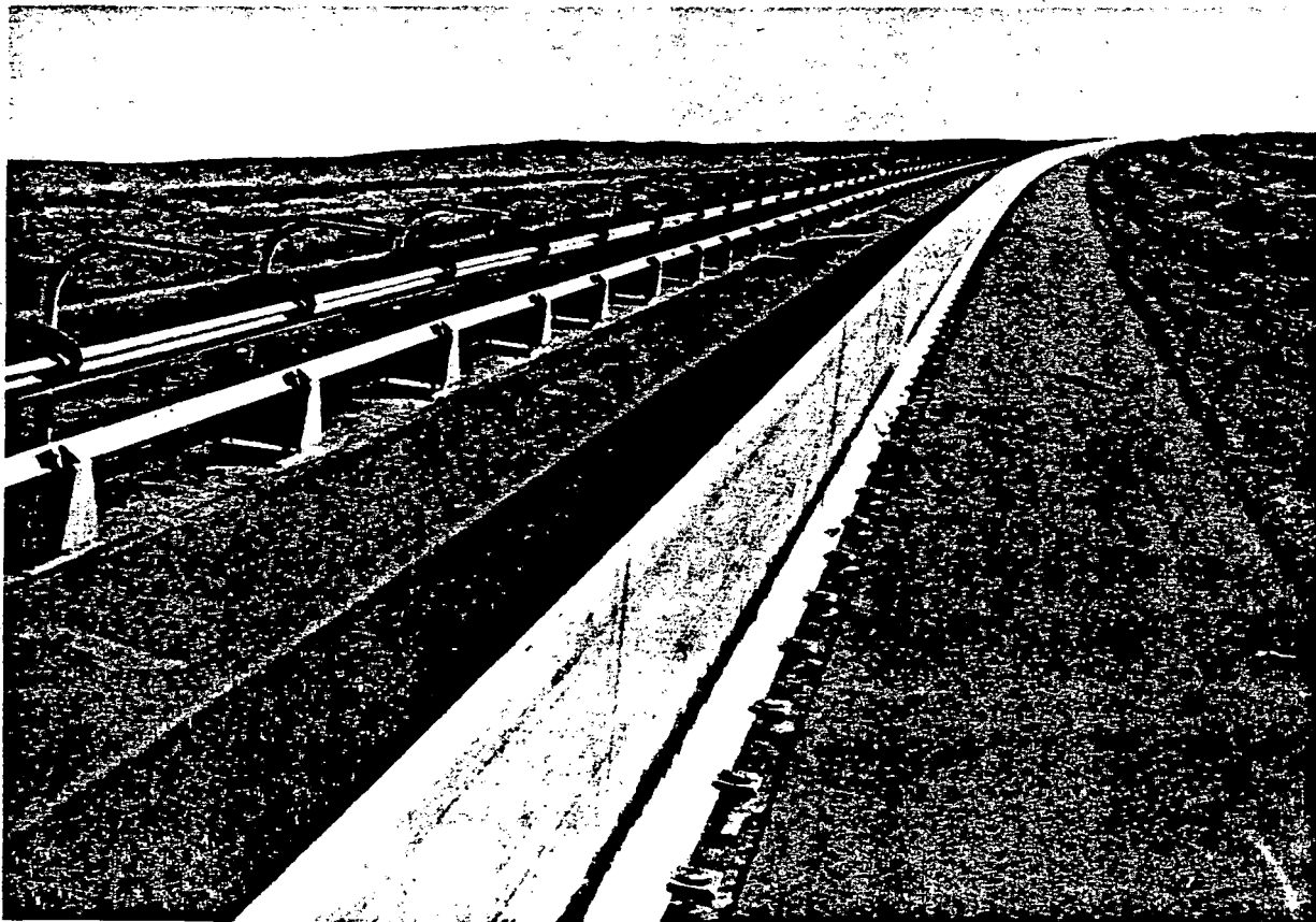
Figure 8. PTACV Guideway at Transportation Test Center. Reaction Rail in Center and Power Distribution Rails on Left.
