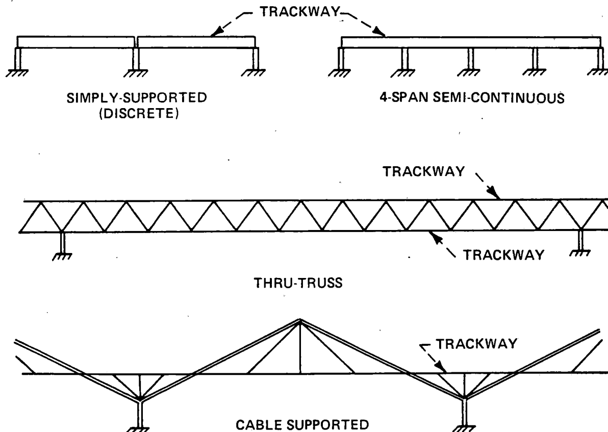
Figure 14. Elevated Guideway Design Concepts
