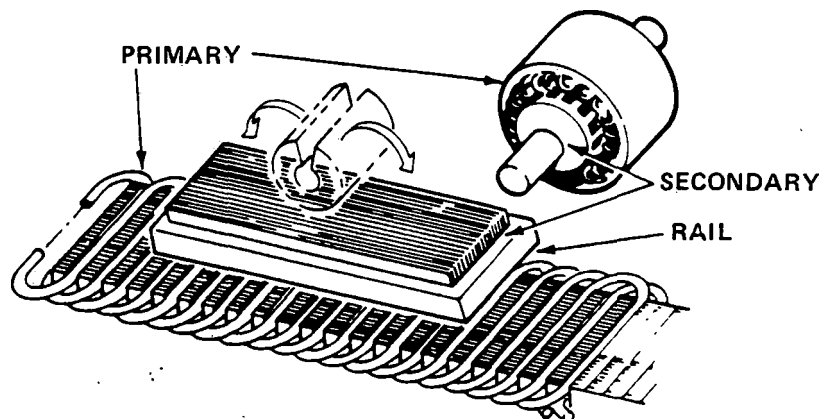
Figure 10. Principle of Single-Sided Linear Electric Motor
