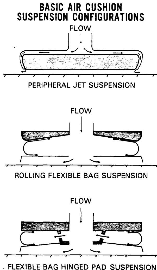
Figure 2. Different Designs of Air Cushion
